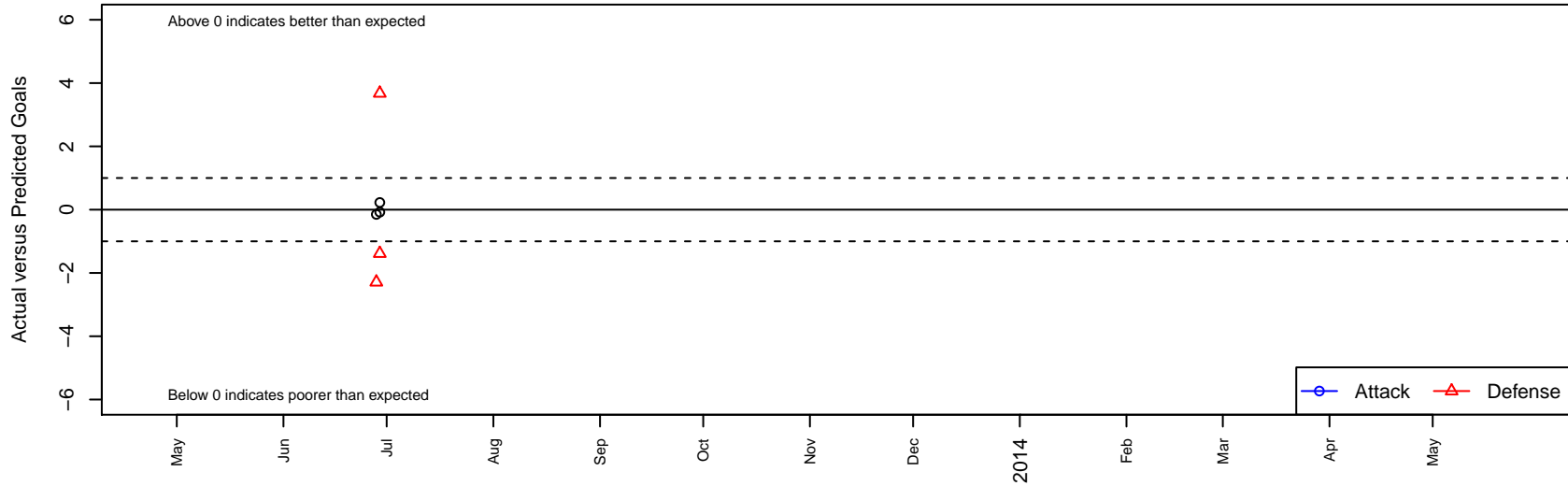
Havoc G00 Dots are actual minus expected GF (blue circles) and GA (red triangles). Blue line is smoothed change in attack strength. Red is smoothed change in defense strength.
